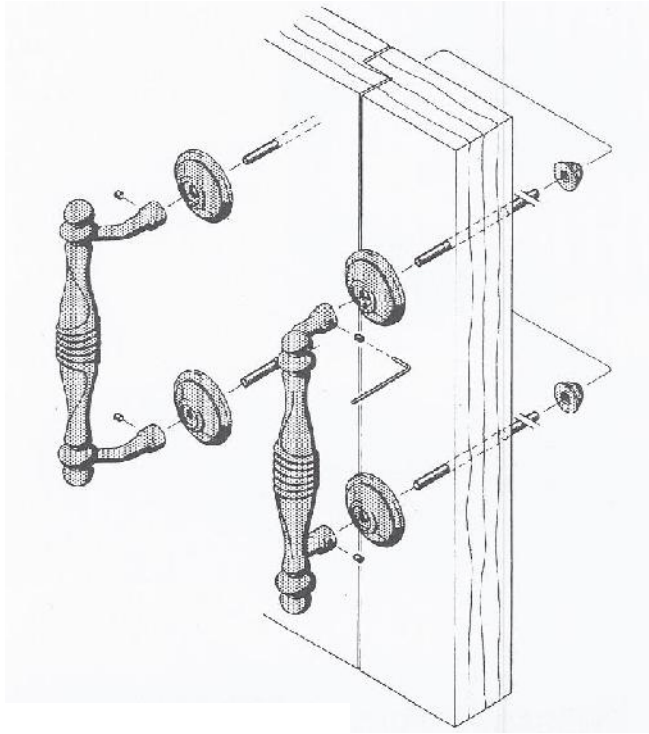
Thru-Bolted Installation
